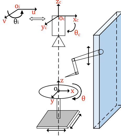
Fig. 3. Configuration of the Robotic Cell Injection Systems
