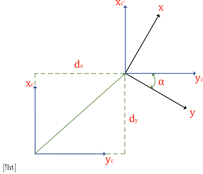
Fig. 4. Transformation from Camera to Stage Coordinate Frames
