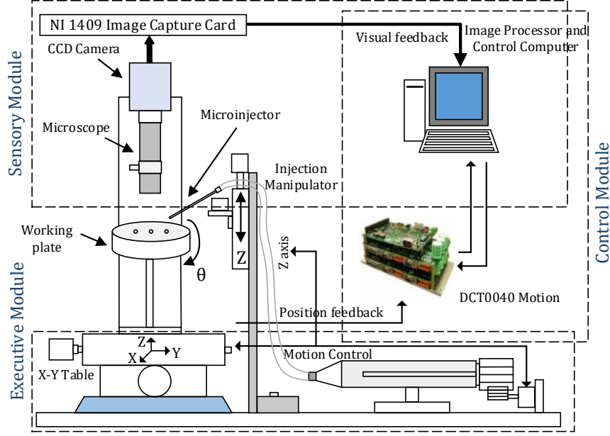
Fig. 2. Robotic Cell Injection Systems
